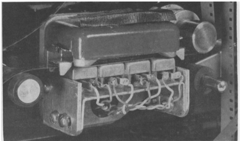
Fig. 3. Four head sound pick-up, selectable by manual switch.
