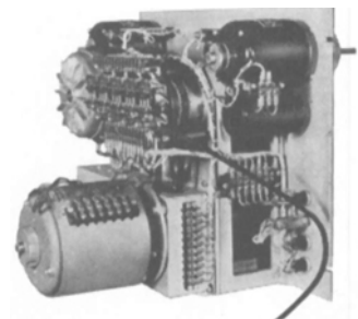
Rear view of transport, showing its compact design, with interlock motor mounted direct to casting of mechanism, at lower left
