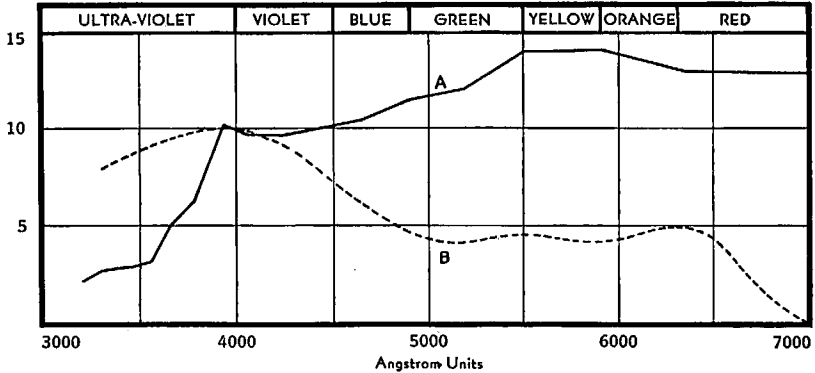
Curve A—Energy Distribution from the new 40 ampere Studio Carbon Arc Curve B—Color Sensitivity of Supersensitive Panchromatic Motion Picture Film
