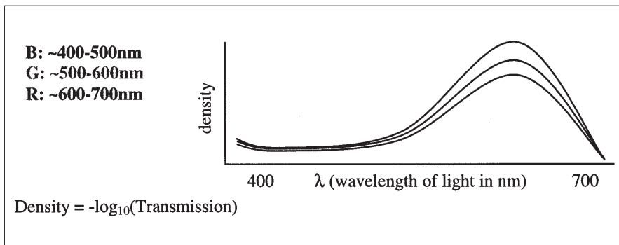
Figure 2. Typical spectral dye density curve for a photographic dye.
