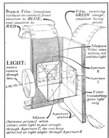
Technicolor 3-strip camera beam splitter, page 496
