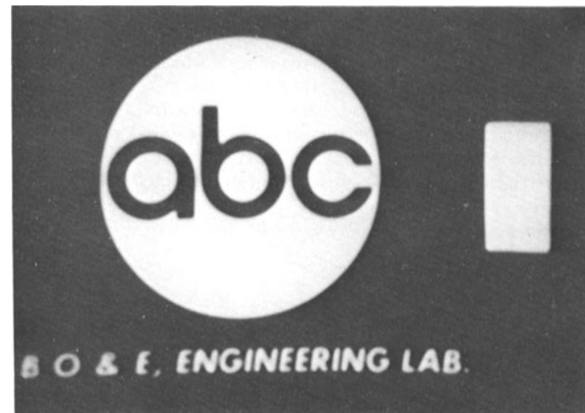
Fig. 2. Waveform and picture monitor displays of a live camera signal distorted within limits of Edmonds' graticule.
