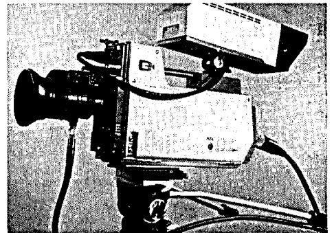
MNC-71CP with 5" viewfinder, mounted on Universal 2030 fluid head tripod (equipped with double handles). Also shown: Remote Production Control Unit and Remote Control Panel ("Paint Box"), camera case and related accessories.
