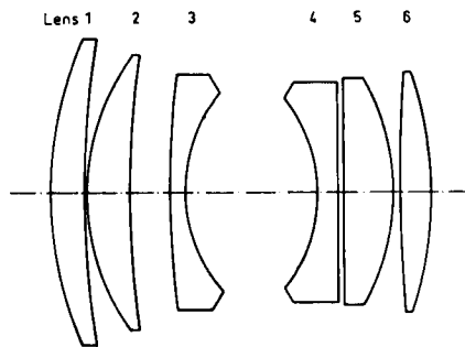
Fig. 1. Cross section of the Super-Kiptar f/2.0 .
