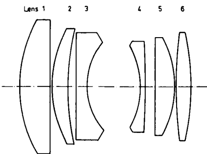
Fig. 2. Cross section of the Cinelux-Ultra f/2.0 .
