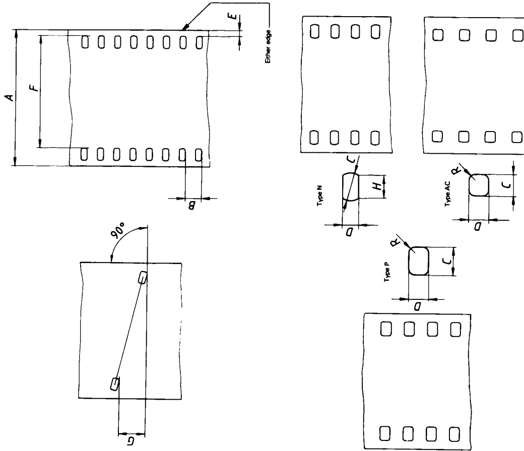
Figure — Types of perforations
