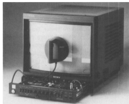
Sony BKM-2052 automatic setup device
