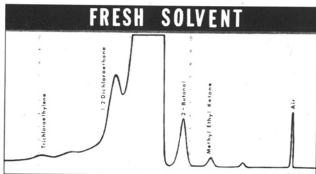
Typical chromatograms of fresh solvent and recovered solvent; all impurities are below the level of 0.1% • A System for the Recovery of Solvent Vapors • E. H. Reichard • JSMPT, July 1963.
