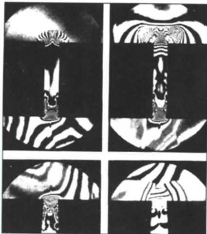
Interferometer pictures of a shock passing through a parallel-walked channel, upper pair, and through a divergent channel, lower pair • Comments on Light Sources • H. E. Edgerton • JSMPT, July 1963.
