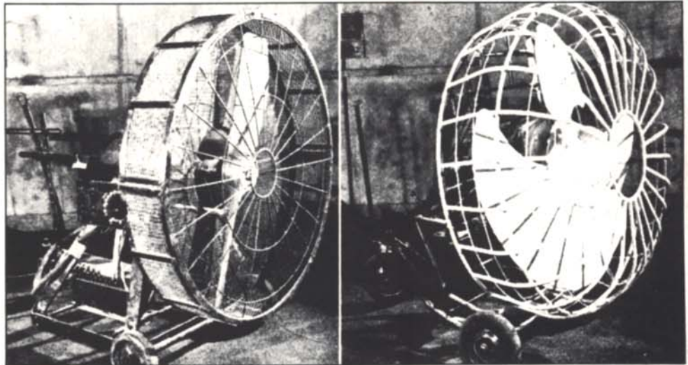
(Left) Airplane type of propeller, with two blades; (Right) Improved 3-blade screw type propeller • Silent Wind-Machine • F. G. Albin • JSMPE , April 1939.
