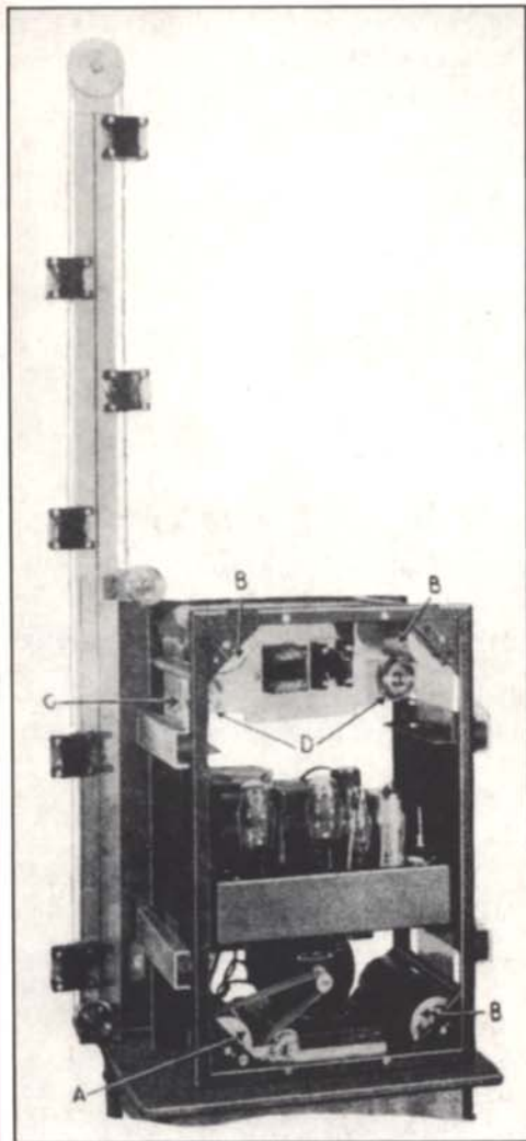
(Top) Mountings for microphone and phototube pre-amplifiers; (Bottom) Mechanism for driving the tape • A Motion Picture Dubbing and Scoring Stage • C. L. Lootens, D. J. Bloomberg, and M. Rettinger • JSMPE , April 1939.
