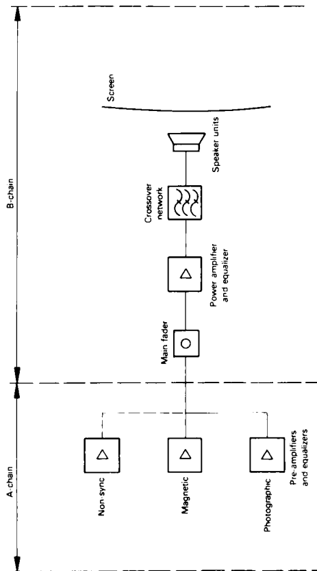
Figure 1 — Complete theatrical sound reproducing system
