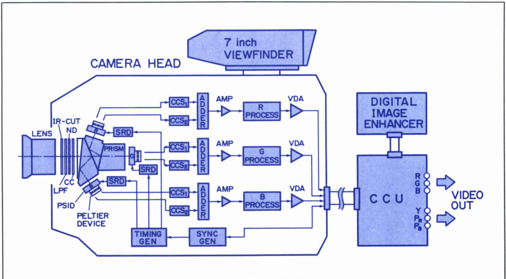
Block diagram of the HDTV color camera.
