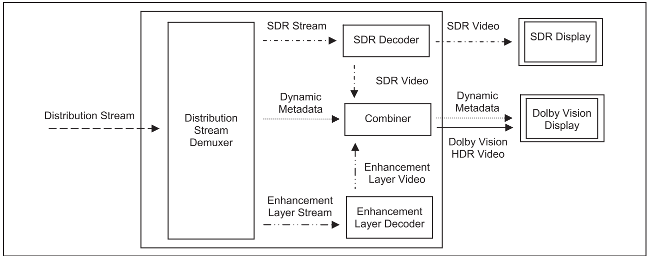
FIGURE 4. The Dolby Vision codec architecture with SDR base layer and HDR enhancement layer.
